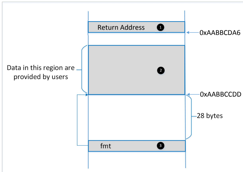
Figure 1: Stack Layout for Problem 6.5.
