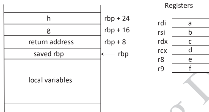
Figure 4.10: Stack layout for the function func()
