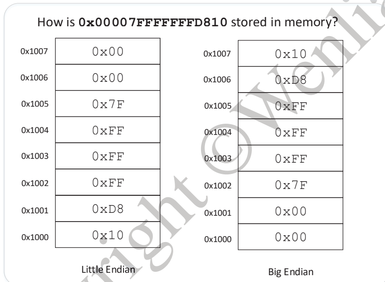
Figure 4.11: Endianness
